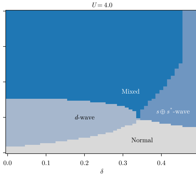
SC and normal regions ( t = 1.0 , L = 256 , \beta = 100.0 )
